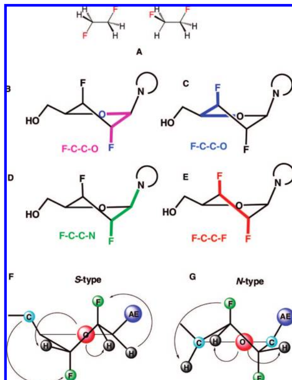
Figure 2. Depiction of the gauche and antiperiplanar effects. In (A), the F atoms in difluoroethane can orient either antiperiplanar (left) or gauche (right). (B–E) Atoms involved in the potential gauche effects in the difluoronucleosides studied in this work; atoms involved are highlighted in bold. Potential antiperiplanar effects (depicted by arrows) for S-type (F) and N-type (G) puckers.
