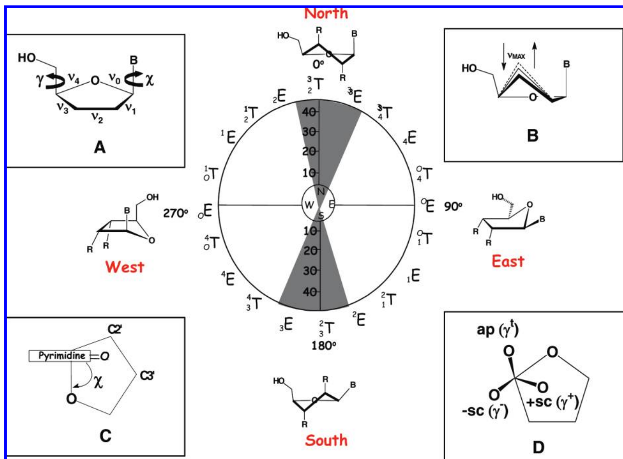
Figure 1. Structural parameters for nucleosides. The pseudorotational cycle (center) describes the ring pucker of the furanose system where the endocyclic torsion angles (shown as \nu_0 – \nu_4 in A) are varied systematically around a “wheel” of twist and envelope conformations. The maximum out-of-plane pucker ( \nu_{\max} , in B) indicates degree to which a specific atom in the five-membered ring will flex from the plane of the five atoms. Angles \chi (C) and \gamma (D) describe the rotamer distribution about the anomeric and C4′–C5′ bonds, respectively.
