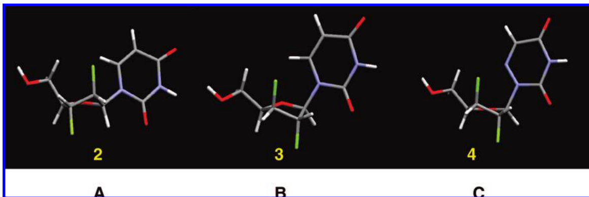
Figure 3. Crystal structures of compounds (A) 2 , (B) 3 , and (C) 4 .
